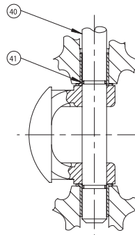
Bearing Seal Construction
