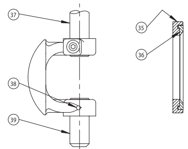
Soft Seat Construction Inseparable Assembly
