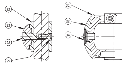
Ceramic or Alloy 6 Plug Construction 1 Inch Valves
