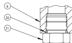
Bottom Plug Construction 1 - 1.5 Inch Valves
