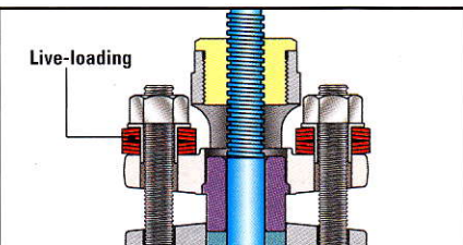
Live-loading
