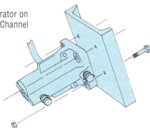
Optional APR Vibrator with Rectangular Mounting Base Plate on APR-M Mounting Channel
